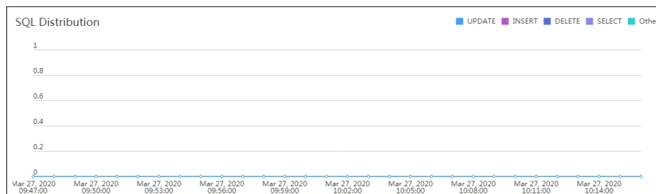
Figure 6-3 SQL distribution
