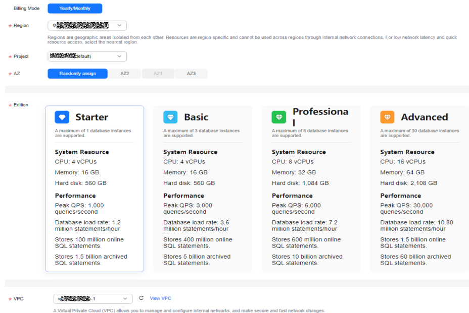
Figure 3-2 Selecting an AZ and an edition
