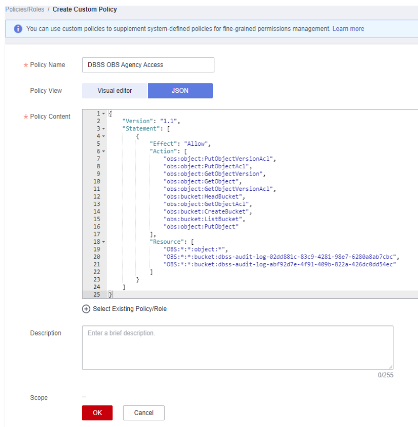
Figure 9-1 Creating a custom policy
