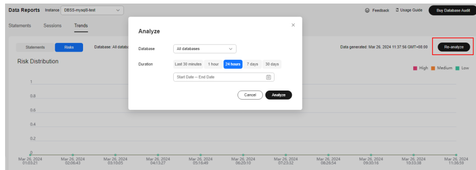
Figure 6-7 Re-analyze
