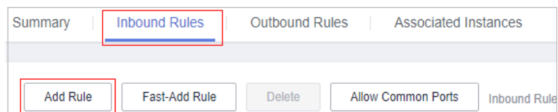
Figure 2-29 Adding rules
