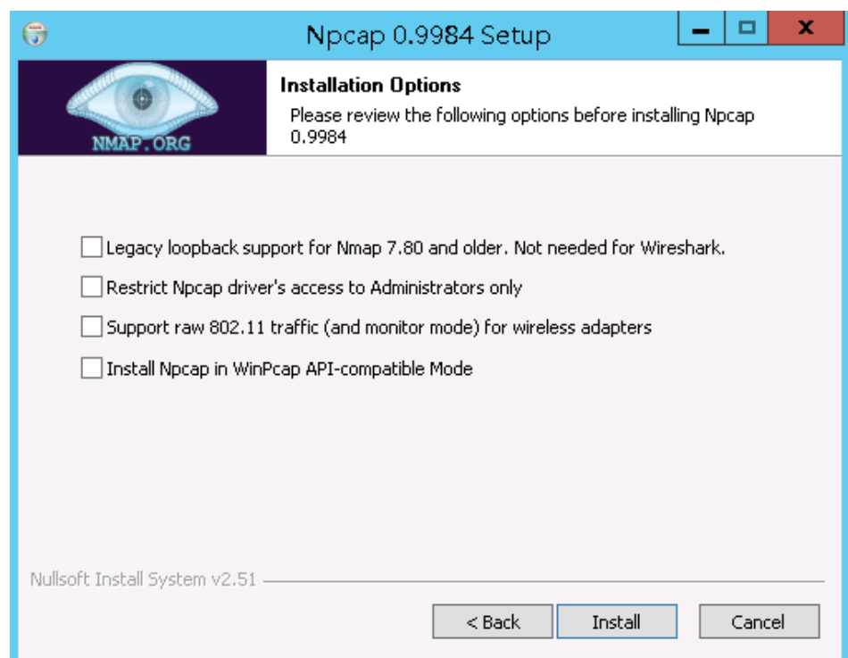
Figure 2-25 Installing Npcap
